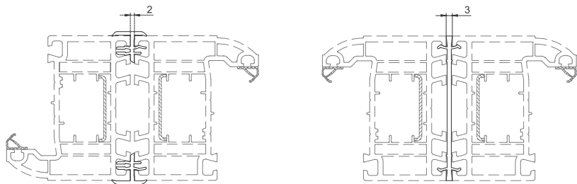
120224 - Coupling Single Sided 140203 - Coupling Full Width (white only)
