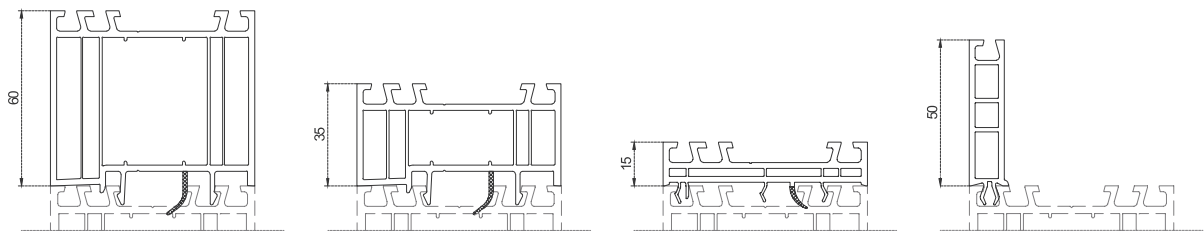
140207 - Frame Extension 60mm 140205 - Frame Extension 35mm 140209 - Frame Extension 15mm 120102 - Single Leg Extension 50mm
