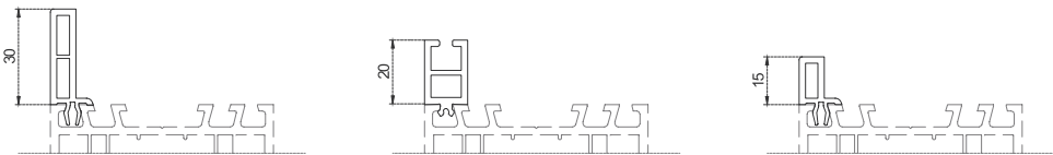
120237 - Single Leg Extension 30mm 120106 - Single Leg Extension 20mm 120236 - Single Leg Extension 15mm
