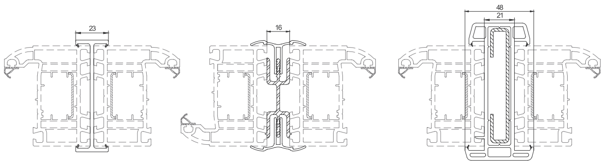
140267 - Coupling Full Width 209044 + 2x 100270 - Multi Vista Coupler 140218 (229018) - Structural Coupling
