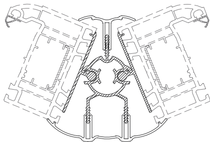
Variable Angle Bay Post (209041) + Adapters (209042) + covers (100270 + 100271)
